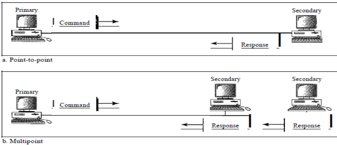
Figure 11.25 Normal response mode
