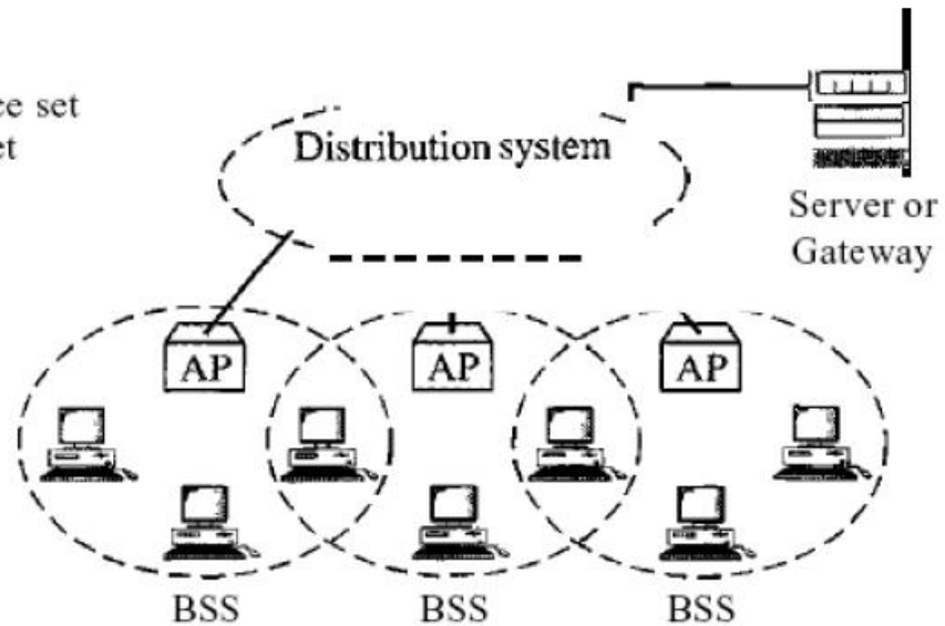
Figure 10 Extended service sets (ESSs)
