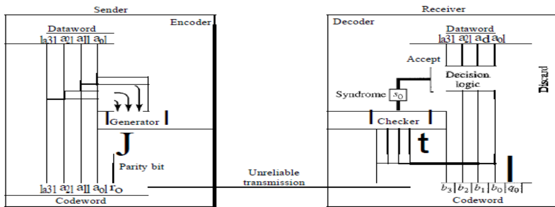
Figure 10.10 Encoder and decoder for simple parity-check code
