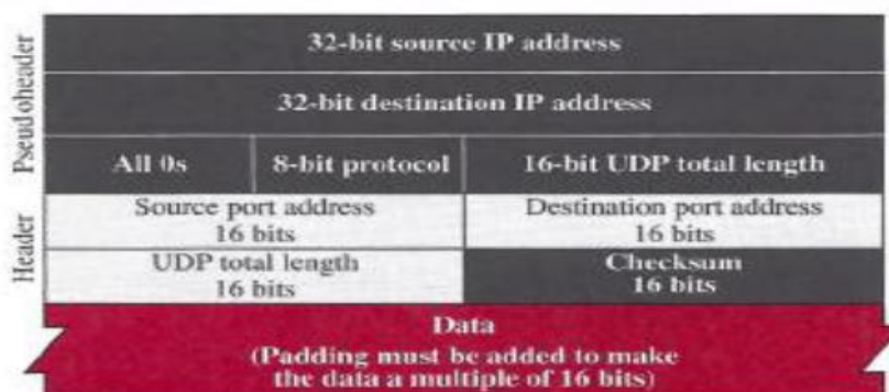
Pseudoheader for checksum calculation
