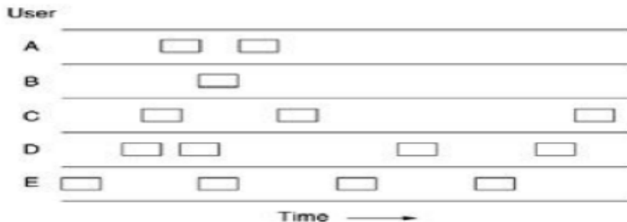
Fig.1 In pure ALOHA, frames are transmitted at completely arbitrary times.
