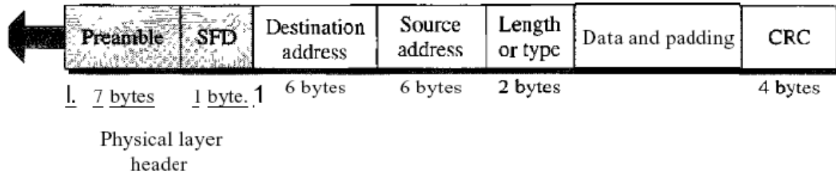
Figure 4 802.3 MACframe
