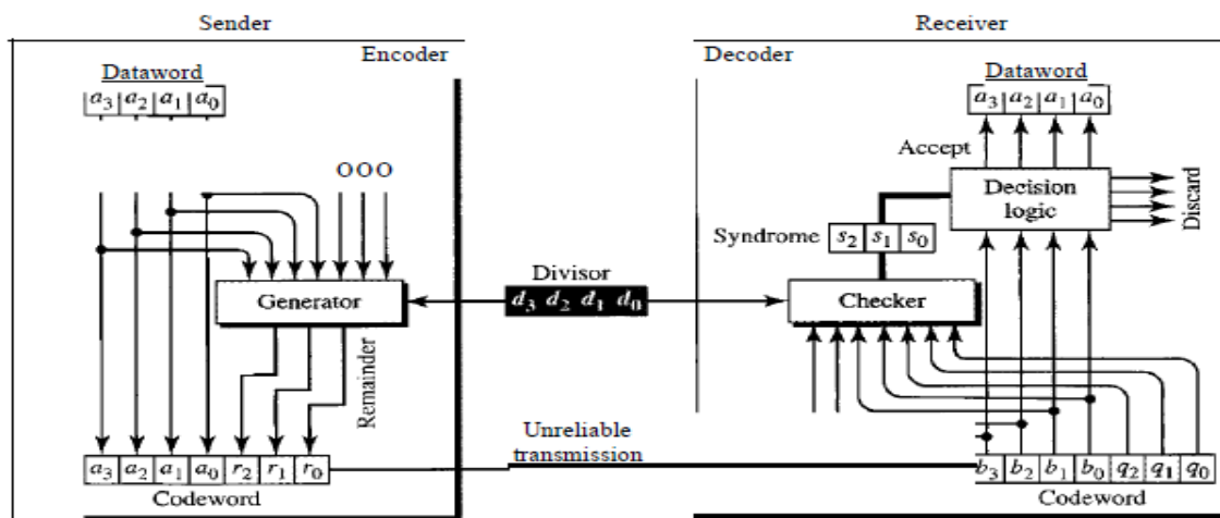
Figure 10.14 CRC encoder and decoder
