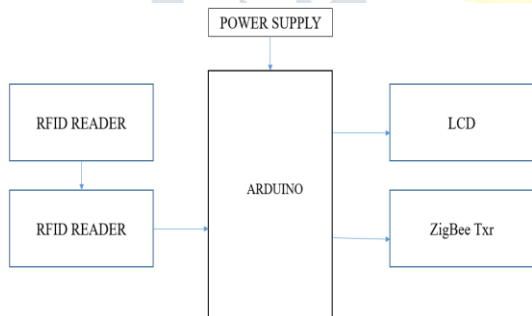
Fig b. Block Diagram
